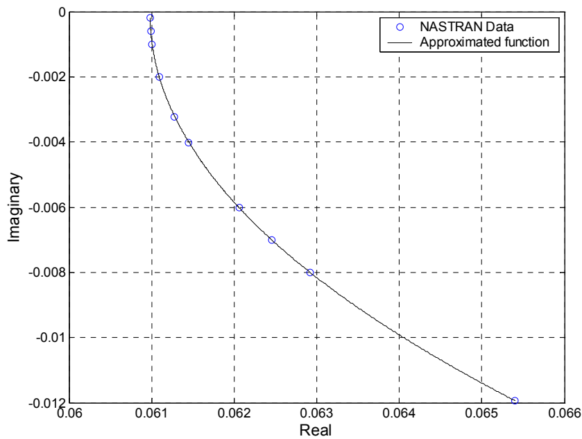
Figure 4. Approximation of Q(2,2) by Roger's approximation
