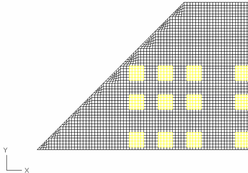
Figure 2. Finite element model of the smart fin
