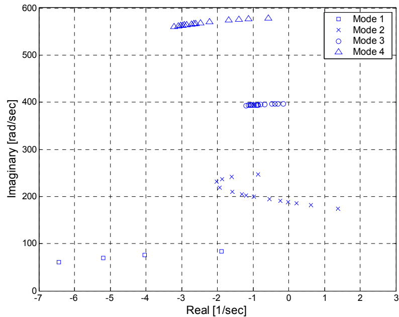
Figure 5. Root-locus of the state-space model of the smart fin as a function of the flight velocity
