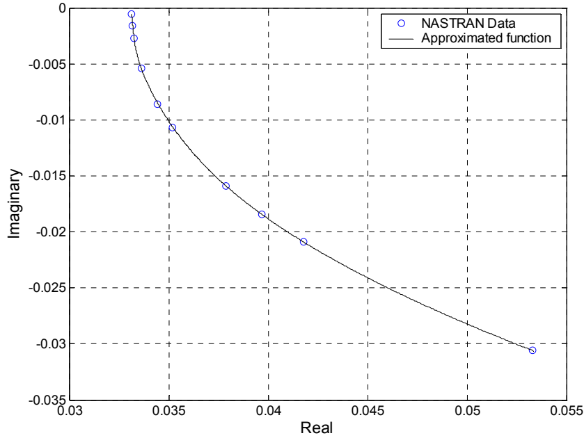
Figure 3. Approximation of Q(1,1) by Roger's approximation
